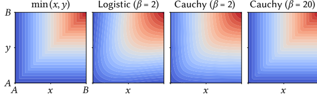
Fig. 3. We visualize different smooth relaxations of the hard minimum operator \min(x, y) for pairs (x, y) \in [A, B]^2 with different stiffness \beta = 1/\tau . The logistic relaxation approximates the minimum but is nonmonotonic, which is undesirable. The Cauchy relaxation offers a monotonic alternative with bounded error, which can be “hardened” by progressively decreasing the temperature parameter \tau to improve the approximation.
