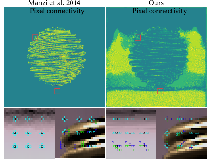
Fig. 6. Comparison between the number of pixels connected and the shape of the kernel between Manzi et al. [2014] and ours. Our method favors unstructured kernels in smooth areas and adapts to local features when required. Cyan indicates bidirectional selection, whereas blue and green mean forward and backward selections.
