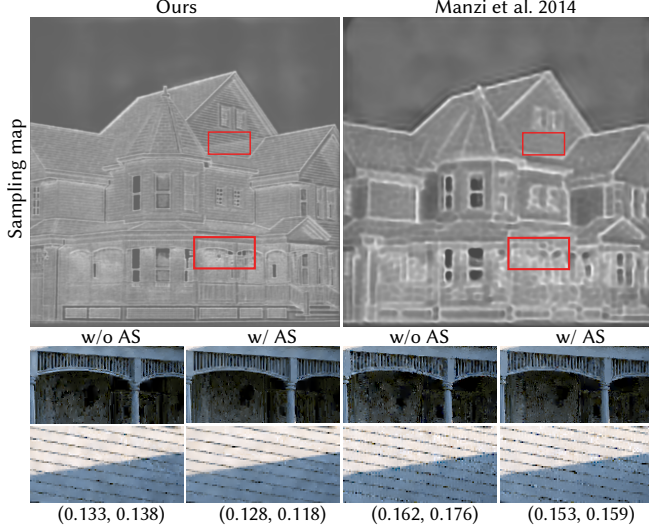
Fig. 7. Comparison of adaptive sampling with and without it for SAK [Manzi et al. 2014] and our method. We see comparable sampling patterns, but our method more effectively distributes samples across the image due to our end-to-end approach.
