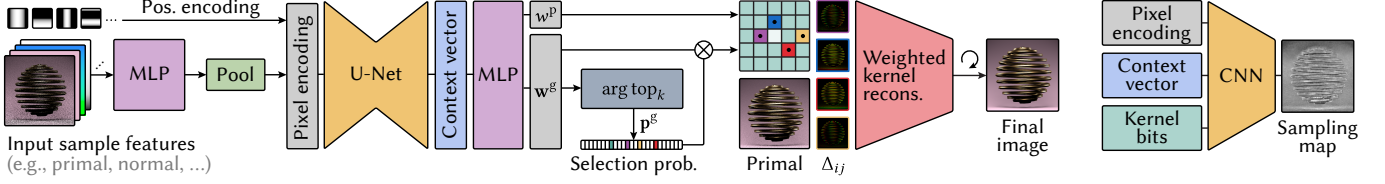
Fig. 4. Pipeline overview. Left: A small per-sample MLP first encodes and aggregates sample features into per-pixel summary statistics. These pixel encodings are then processed by a U-Net to produce a context vector that gets decoded into a weighted neighbor kernel w^g and a primal weight w^p . A differentiable sorting network uses these weights to rank and pick appropriate neighbors for the weighted reconstruction. Right: Our adaptive sampling network uses the encoded inputs, the deep context and the predicted kernel bits to build the sample map that is used to generate I and \Delta_{ij} . The model is trained end-to-end.
