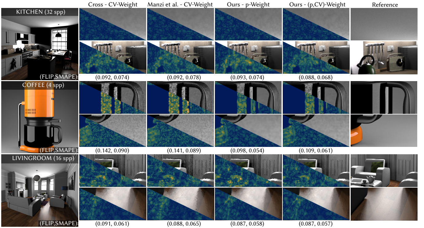
Fig. 11. Comparison between our method and baselines with CV weighted reconstruction [Rousselle et al. 2016] and our method combining our predicted weights and variance statistics ( (p,CV)-Weight ). All regions see reduced reconstruction artifacts when variance statistics are included.
