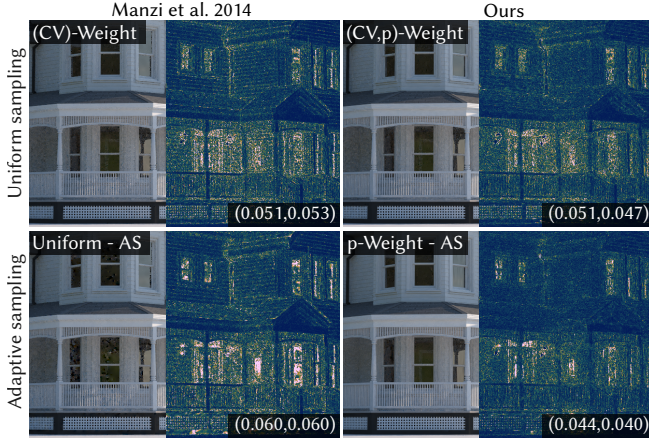
Fig. 9. Comparison of adaptive sampling with and without it for SAK [Manzi et al. 2014] and our method for path tracing integrator. We can observe that our adaptive sampling and kernel adaptation generalize to this integrator. SMAPE Error is visualize here.
