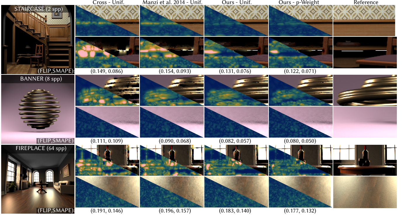
Fig. 10. Comparison between our method and baselines with uniform reconstruction [Rousselle et al. 2016] and our methods of reconstruction using our predicted weights ( p-Weight ). We can see that in all regions, our method reduces dipole artefacts and accurately captures geometrical and shading changes.
