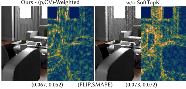
Fig. 5. Comparison with and without differentiable sorting networks (DSNs) for our method. Without DSN, optimization get trap inside a minima which translate to artefacts inside the reconstructed image.
