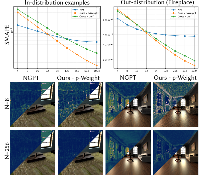
Fig. 8. Comparison between NGPT [Kettunen et al. 2019b] and our method across varying input sample counts. Our method demonstrates improved generalization and is unbiased compared to NGPT.
