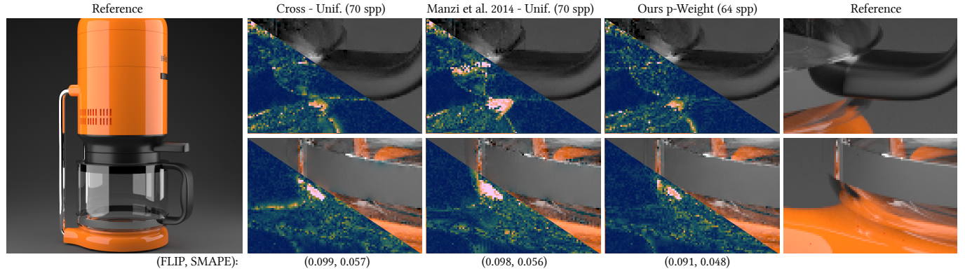
Fig. 1. Equal-time comparison between our adaptive kernel, the structure-adaptive kernel [Manzi et al. 2014], and the standard cross-shaped kernel. All methods use gradients produced by gradient-domain path tracing with path reconnection.
